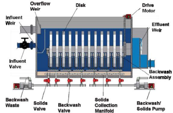
Figure 11-2. Cutaway view of AquaDisk® cloth media filter.
