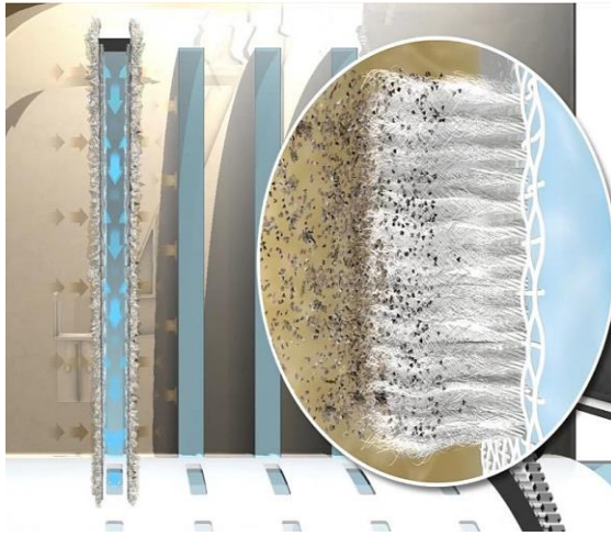
Figure 11-2. Cutaway view of AquaDisk® cloth media filter.
